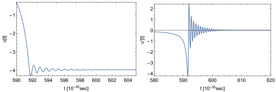
Figure 5. In the left panel—blown-up portion of the plot on Figure 2 around and after end of inflation depicting the oscillations of u(t) after end of inflation. In the right panel—oscillations of \dot{u}(t) after end of inflation.
