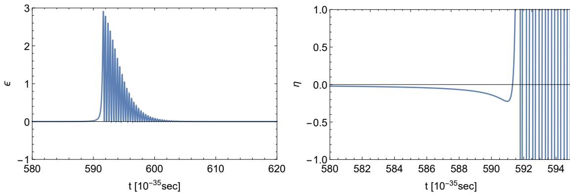
Figure 3. Slow-roll parameters \epsilon and \eta before and around end of inflation. When \epsilon = 1 the inflation ends.
