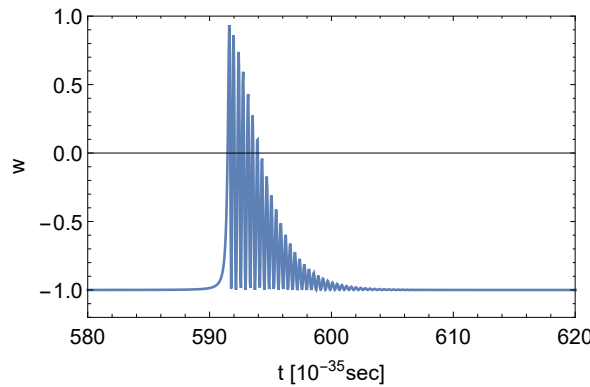
Figure 6. Evolution of w parameter of the equation of state with sharp growth above w \approx -1 for a short time interval after end of inflation—matter domination.
