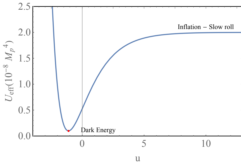
Figure 1. Shape of the effective potential U_{\text{eff}}(u) in the Einstein-frame (37). The physical unit for u is M_{Pl} / \sqrt{2} .
